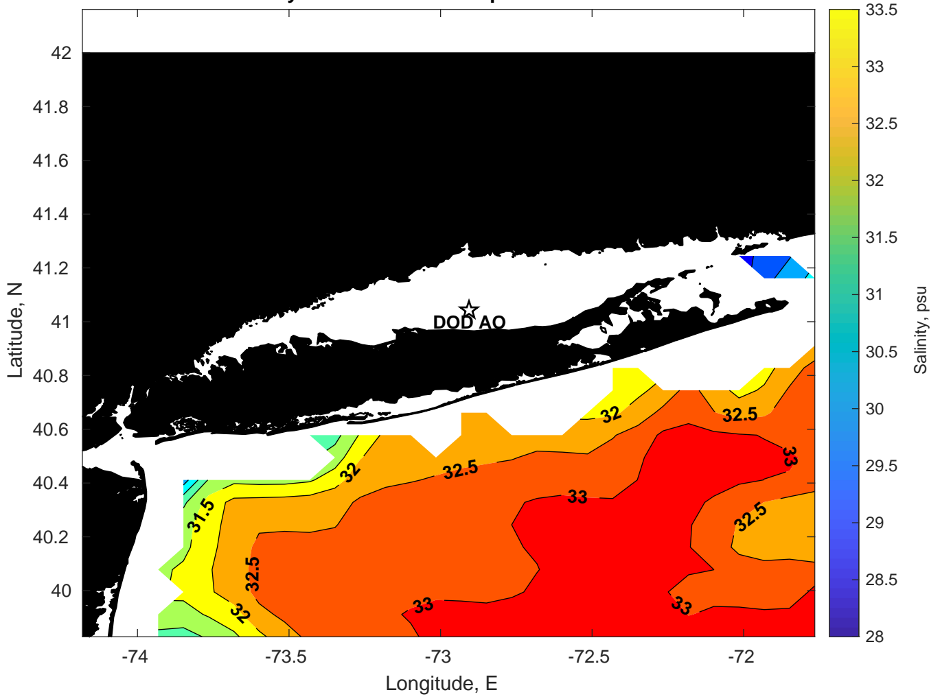
Surface Salinity for DOD AO at 27-Apr-2024 00:00:00
